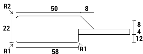
profilo ferma vetro | glass retainer profile
